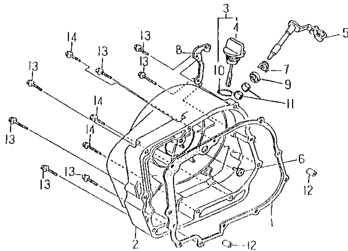
FIG.09 RIGHT CRANKCASE COVER 右曲軸箱蓋
