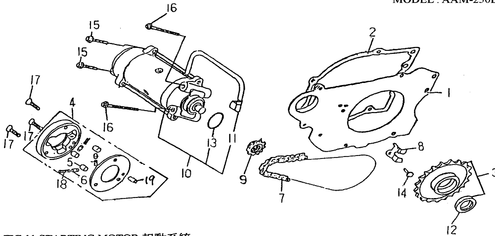
FIG.11 STARTING MOTOR 起動系統
