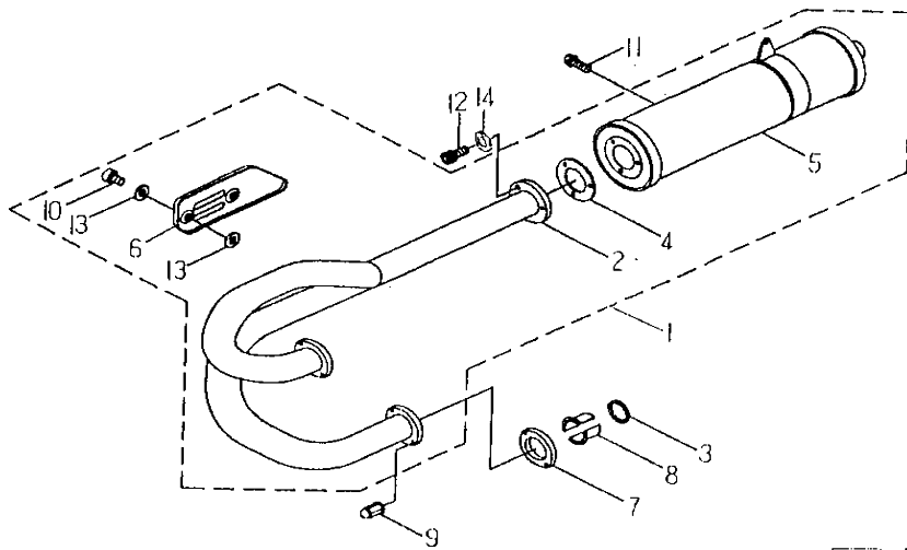
FIG.14 EXHAUST MUFFLER 排氣管
