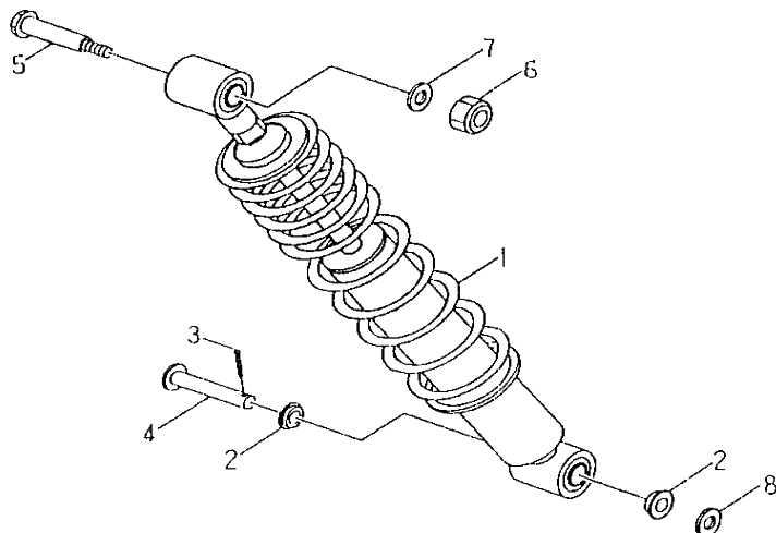
FIG.16 REAR SUSPENSION 後懸吊系統
