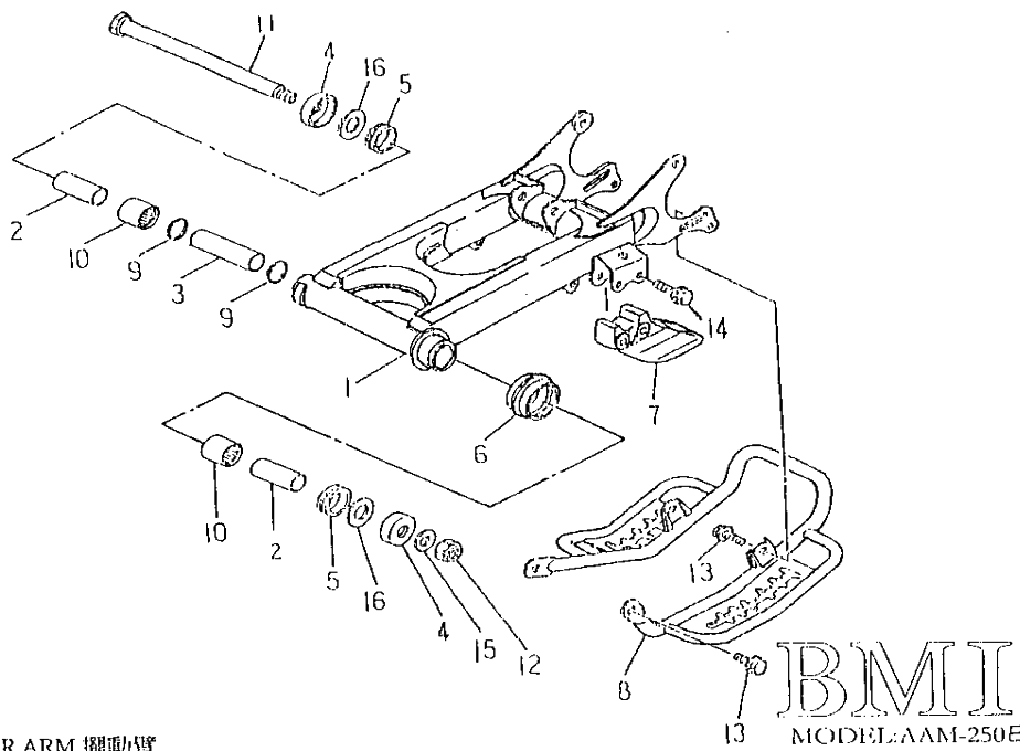
FIG.15 REAR ARM 擺動臂
