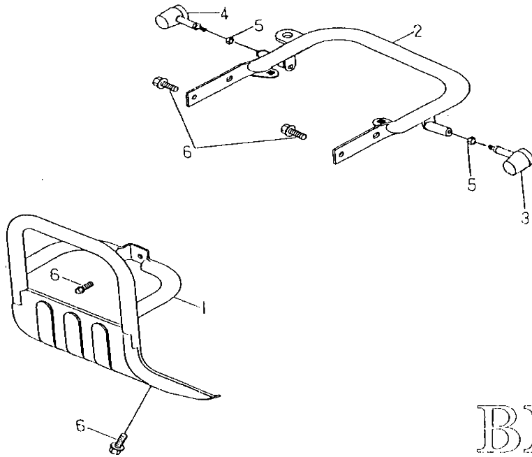
FIG.31 GUARD 保護桿
