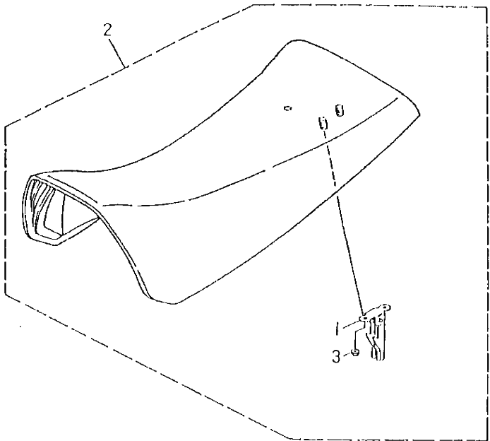
FIG.23 SEAT 座墊
