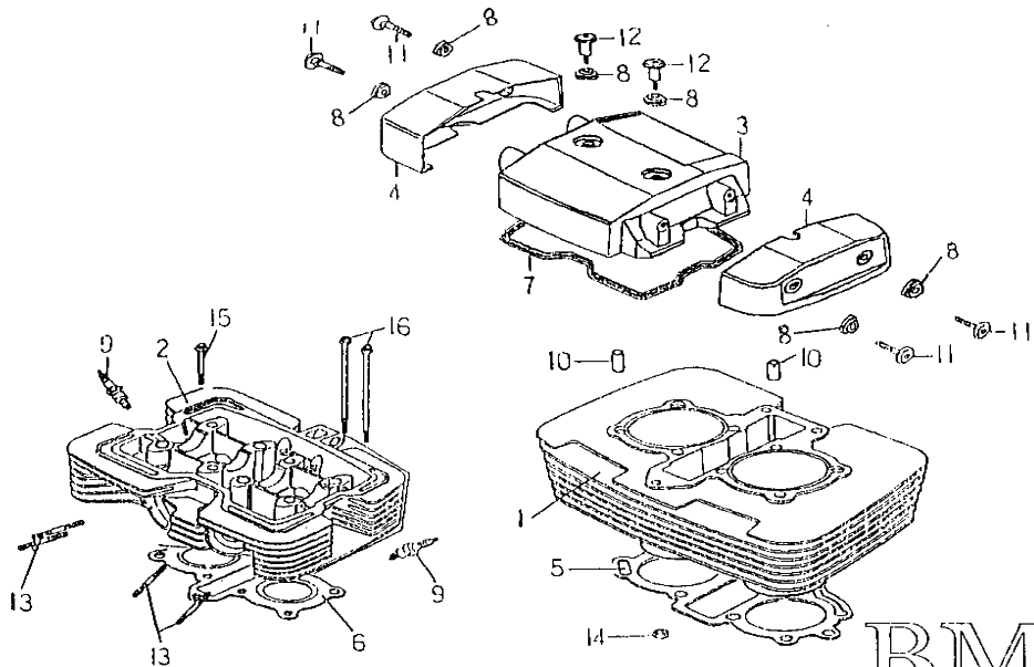
FIG.01 CYLINDER.CYLINDER HEAD 汽缸.汽缸頭
