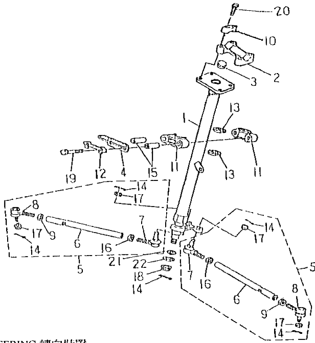
FIG.19 STEERING 轉向裝置
