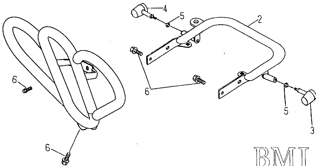
FIG.31 GUARD 保護桿 (FOR OIL COOLER)
