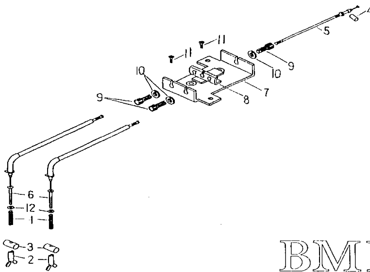
FIG.27 INTEGRATED 整合式制車系統
