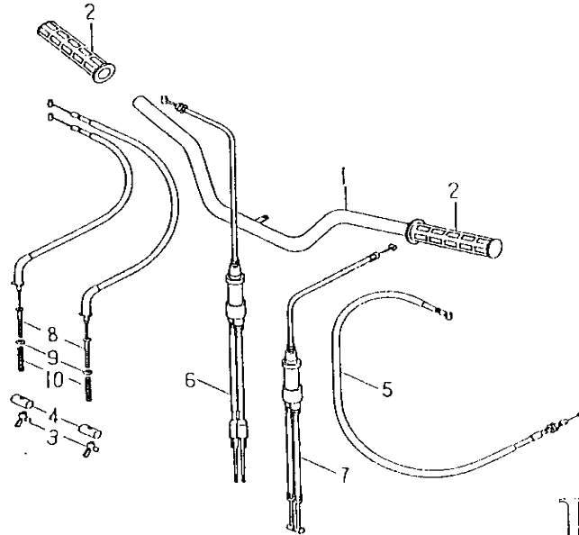
FIG.28 STEERING HANDLE CABLE 轉向把手,鋼索
