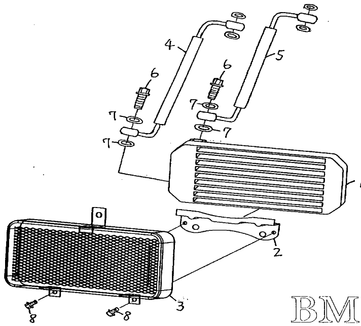
FIG.39 OIL COOLING SET 機油冷卻裝置
