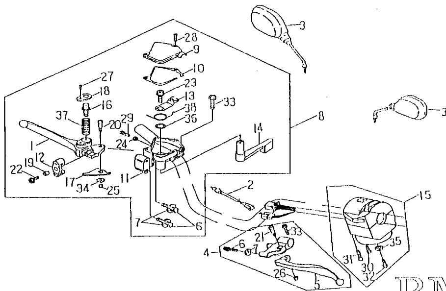
FIG.29 HANDLE SWITCH , LEVER 把手開關,拉桿
