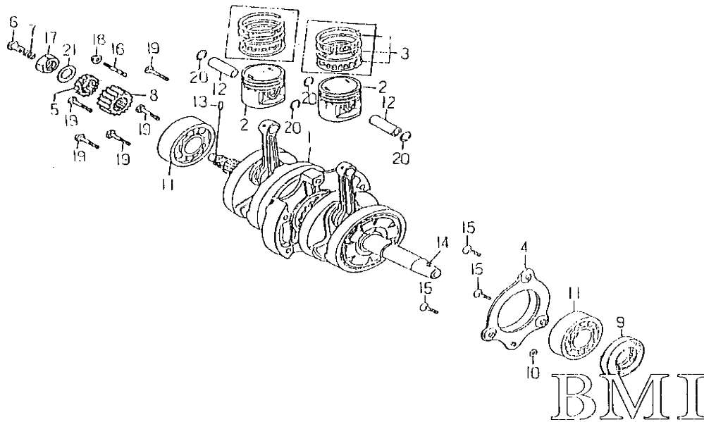
FIG.02 CRANKSHAFT.PISTON 曲轴.活塞
