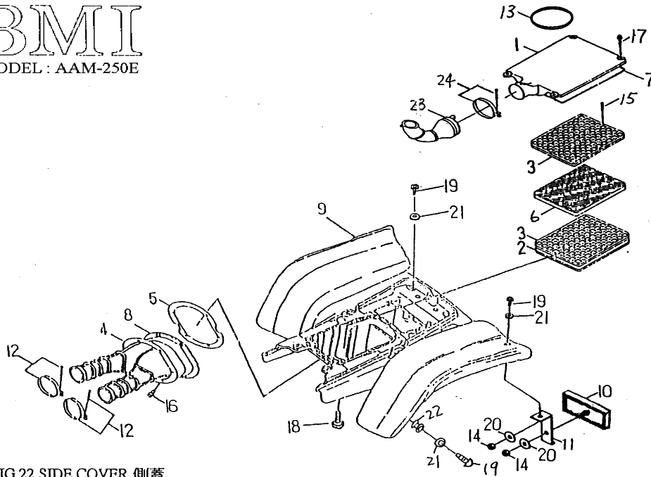
FIG.22 SIDE COVER 側蓋
